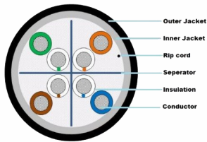
CAT 6 UTP DOUBLE JACKET LAN CABLE
