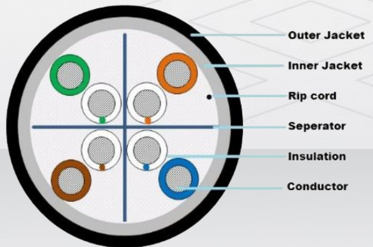
CAT 6 UTP DOUBLE JACKET LAN CABLE
